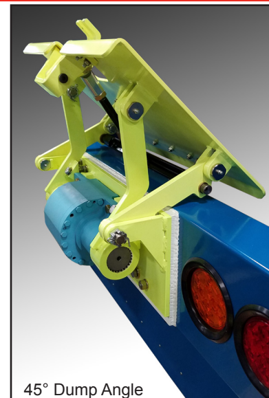
45° Dump Angle
